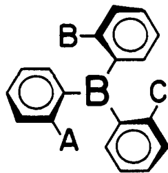
Figure 1. A triarylborane in the propeller conformation.
