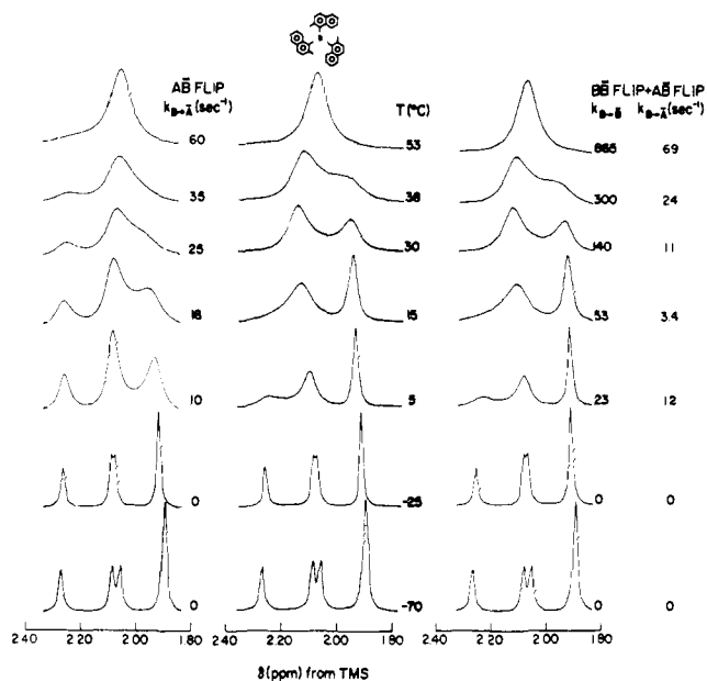
Figure 6. A triptych depicting the 100-MHz ^1\text{H} -nmr spectrum (methyl region) of 1 at various temperatures. The central section displays the experimental spectra. The left-hand panel shows the calculated spectra based upon the \text{A}\bar{\text{B}} -flip alone ( k_{\text{B}\rightarrow\bar{\text{A}}} or k_{\bar{\text{B}}\rightarrow\text{A}} ). The right-hand panel shows calculated spectra for the combinations of the \text{B}\bar{\text{B}} ( k_{\text{B}\rightarrow\bar{\text{B}}} or k_{\bar{\text{B}}\rightarrow\text{B}} ) and \text{A}\bar{\text{B}} -flips which match the experimental spectra (see text).
