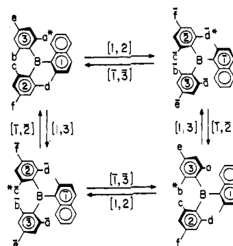
Figure 9. The effect of enantiomeric [1,2]- and [1,3]-flips on the interchange of environments (letters) of a given methyl group (asterisk) in 4 . The aryl ring environments are labeled with numerals, and the numerals along the arrows identify the rings which flip during the specified interconversion. In the text, the flip pathways (undirected) are identified only by the unbarred designations.
