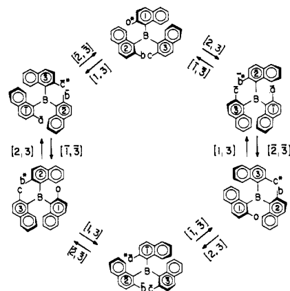
Figure 5. The effect of the enantiomeric two-ring flips on the interchange of environments for a given methyl group in \bar{B}\bar{B}^* (asterisk). Diastereotopic methyl group environments have been labeled with lower case letters, and diastereotopic aryl ring environments have been labeled with numerals. Bared letters or numerals denote enantiomeric relationships. The numerals along the arrows identify the rings which flip during the specified interconversion. Note that since the [1,3]- and [2,3]-flips are enantiomeric, the reverse of the [1,3]-flip, for example, is the [\bar{2},\bar{3}] -flip.
