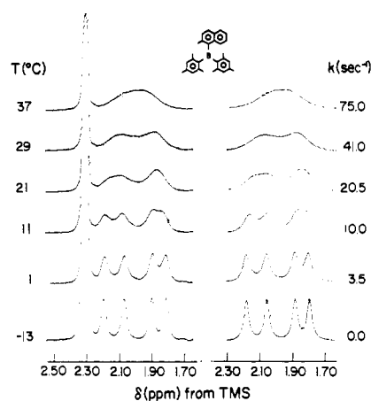
Figure 10. The 60-MHz ^1\text{H} -nmr spectrum (methyl region) of 4 at various temperatures (left), and the corresponding calculated spectra ( o -mesityl methyl portion) based upon the two-ring flip mechanism (right).
