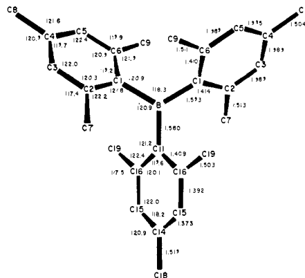
Figure 2. A drawing of a trimesitylborane molecule which depicts bond lengths to the right of the crystallographic twofold axis and bond angles to the left of this axis. The standard deviations of the bond lengths are \leq 0.004 Å in all cases.
