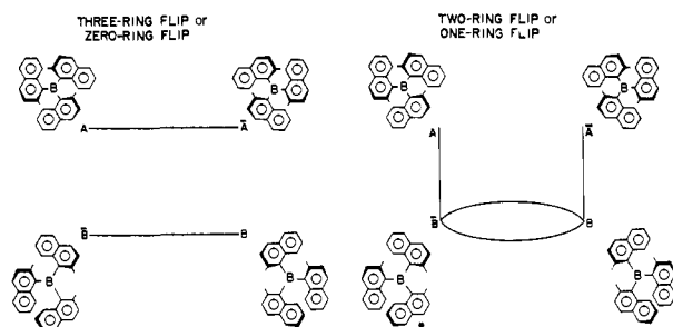
Figure 4. Graphs depicting stereoisomerization of 1 by the flip mechanisms.
