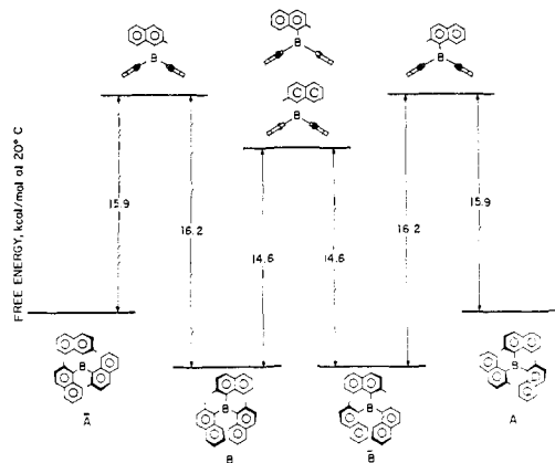
Figure 7. A schematic representation of the energetics of stereoisomerization of 1 . The black circles projecting toward (solid circle) or away from (broken circle) the observer represent methyl groups.
