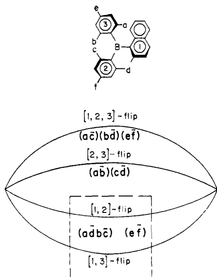
Figure 8. Graph depicting enantiomerization of 4 by two- and three-ring flips. The methyl group environments have been labeled with lower case letters, and barred letters designate enantiomeric relationships. The site exchange ( a\bar{d}b\bar{c} ) signifies that the methyl group is carried from environment a into \bar{d} , etc.
