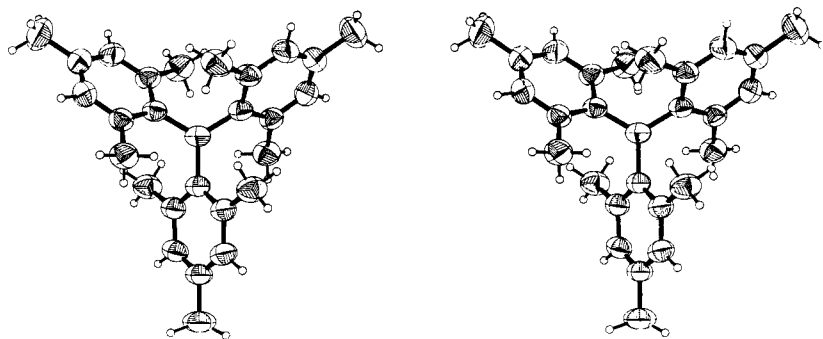
Figure 3. A stereoview of a trimesitylborane molecule. The crystallographic twofold axis passes through the vertical B-C bond. The thermal ellipsoids of the non-hydrogen atoms are scaled to 50% probability. The hydrogens are shown as spheres of arbitrary size.
